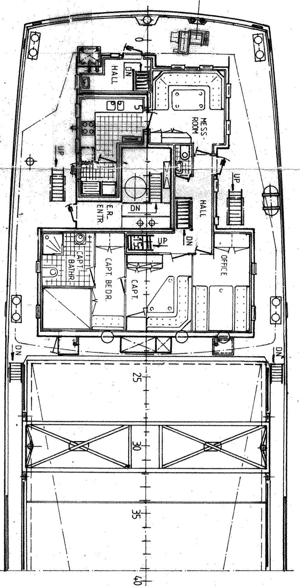
POOPDECK / KAMPAGNEDECK (1-7450/7530)
