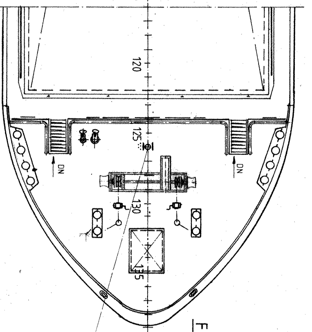
FORCASTLEDECK BAKDECK (1-8650)
