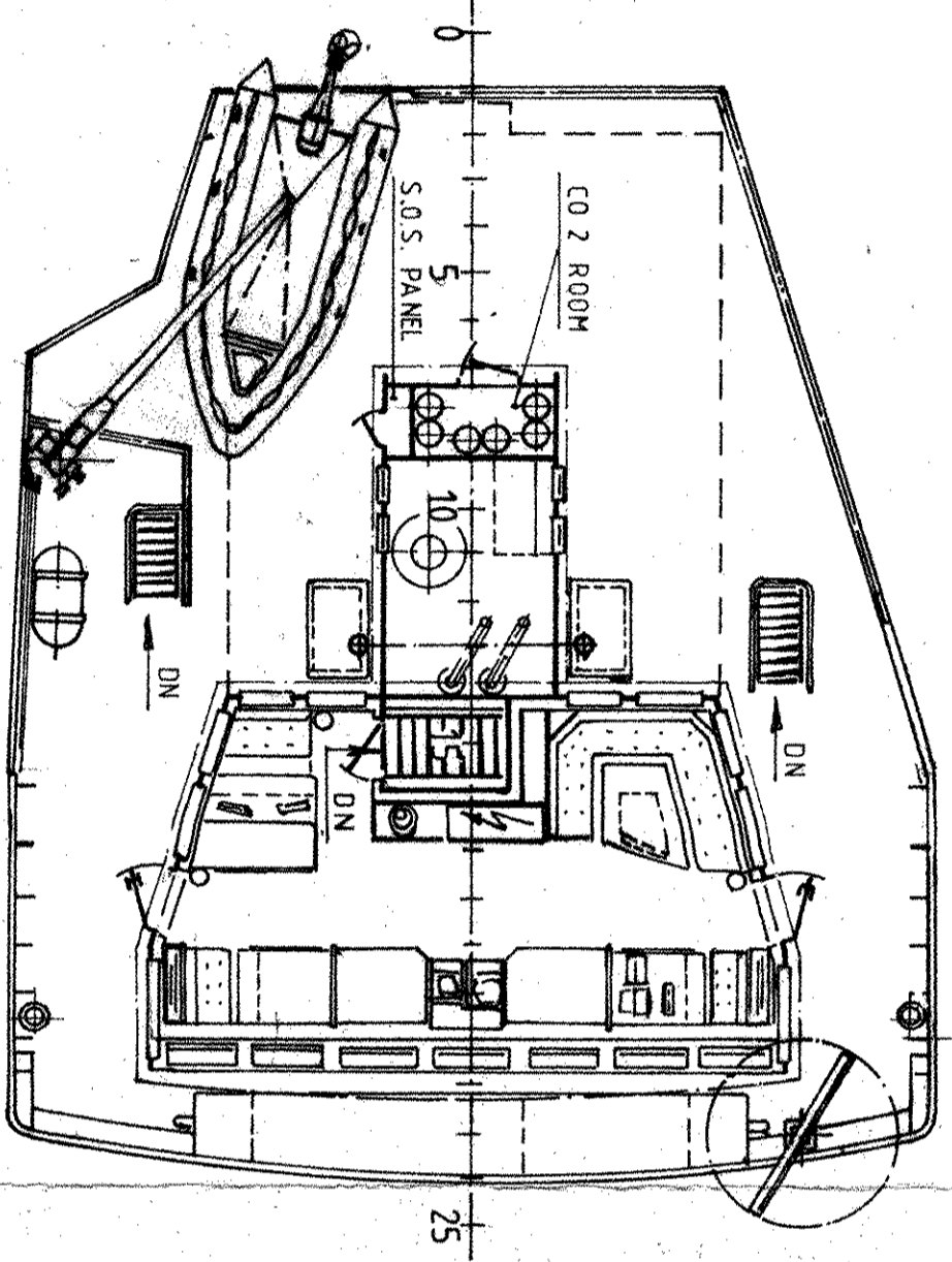
BRIDGE DECK BRUGDECK (1-10000)
